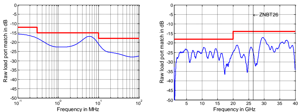
Raw load port match versus frequency for the R&S®ZNBT26/R&S®ZNBT40
